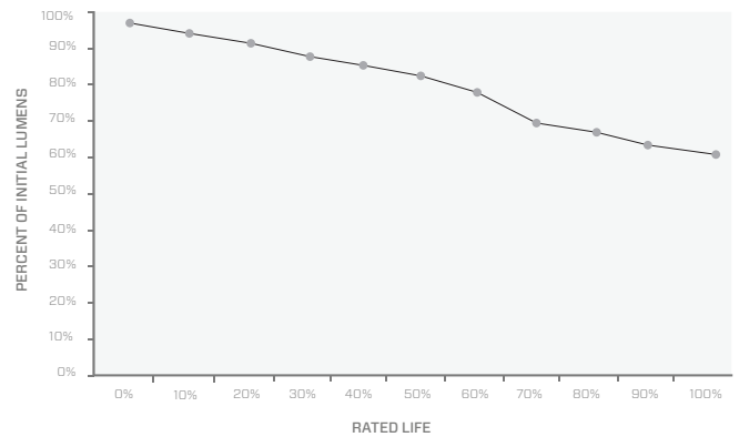
2.2 - LUMEN MAINTENANCE
